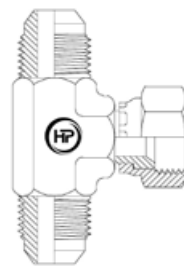
JICM X JICM X JICF BRANCH TEE
