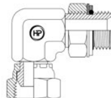
BSPPM X BSPPF 90° ELBOW (M X FS)
