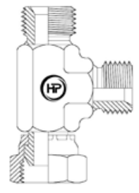
BSPPM X BSPPF X BSPPM RUN TEE
