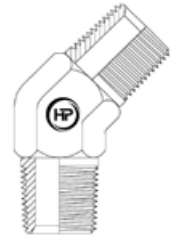
BSPTM X BSPTM 45° ELBOW (M X M)
