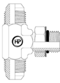
JICM X JICM X UNOM BRANCH TEE
