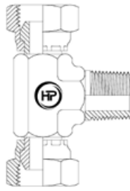
BSPPF X BSPPF X BSPTM BRANCH TEE
