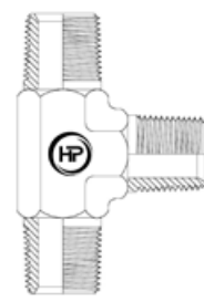
BSPTM X BSPTM X BSPTM EQUAL TEE
