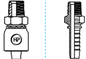
BSPT MALE STRAIGHT
