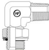
BSPTM X BSPPM 90° ELBOW (M X M)
