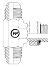
JICM X JICM X BSPPM BRANCH TEE
