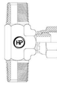
BSPTM X BSPTM X BSPPF BRANCH TEE
