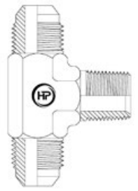
JICM X JICM X BSPTM BRANCH TEE
