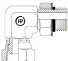
UNOM X BSPPF 90° ELBOW (M X FS)
