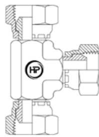
BSPPF X BSPPF X BSPPF EQUAL TEE
