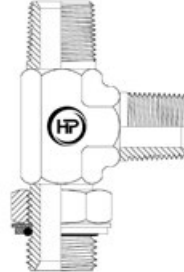
BSPTM X BSPPM X BSPTM RUN TEE
