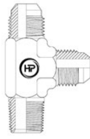
JICM X BSPTM X JICM RUN TEE
