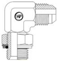
JICM X BSPPM 90° ELBOW (M X M)
