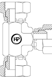
BSPPF X BSPPF X BSPPF EQUAL TEE
