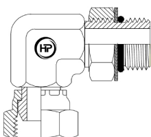
UNOM X BSPPF 90° ELBOW (M X FS)
