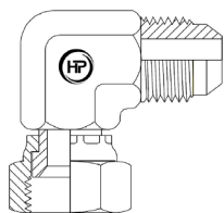
JICM X JICF 90° ELBOW (M X FS)
