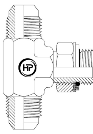
JICM X JICM X BSPPM BRANCH TEE
