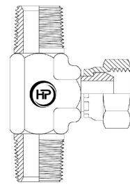
BSPTM X BSPTM X BSPPF BRANCH TEE
