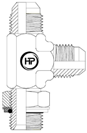
JICM X BSPPM X JICM RUN TEE
