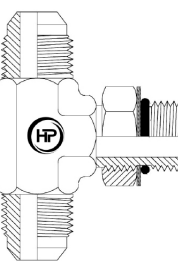
JICM X JICM X UNOM BRANCH TEE
