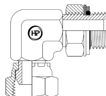
BSPPM X BSPPF 90° ELBOW (M X FS)
