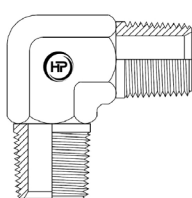
BSPTM X BSPTM 90° ELBOW (M X M)
